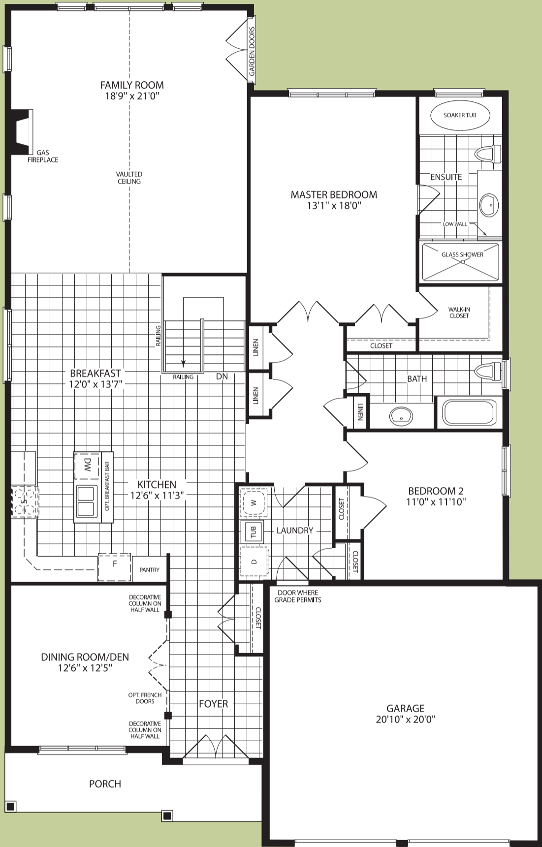
MAIN FLOOR OPTION 1
