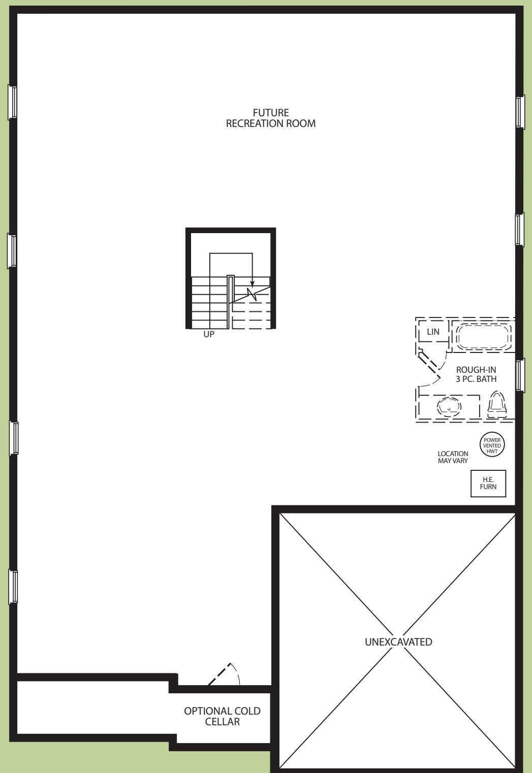
BASEMENT
