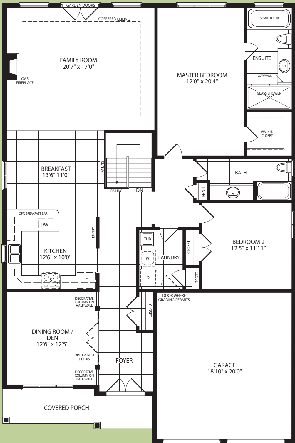
MAIN FLOOR
